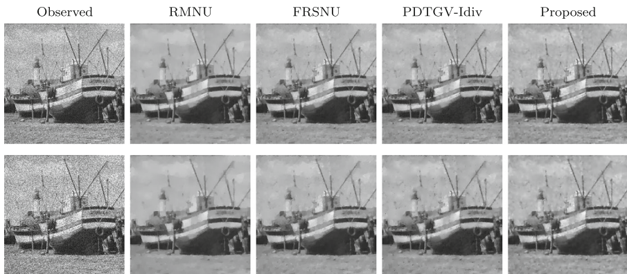
Fig. 7 First row: performance comparison of different methods on Barche with \sigma = 2 , from left to right: observed image, restored results by RMNU with PSNR = 27.54dB , FRSNU with PSNR = 27.87dB , PDTGV-Idiv with PSNR = 27.76dB , and the proposed method with PSNR = 27.96dB ( \lambda = 1.2 , \mu = 10 ). Second row: performance comparison of different methods on Barche with \sigma = 3 , from left to right: observed image, restored results by RMNU with PSNR = 25.64dB , FRSNU with PSNR = 25.96dB , PDTGV-Idiv with PSNR = 25.84dB , and the proposed method with PSNR = 26.17dB ( \lambda = 0.6 , \mu = 50 )
